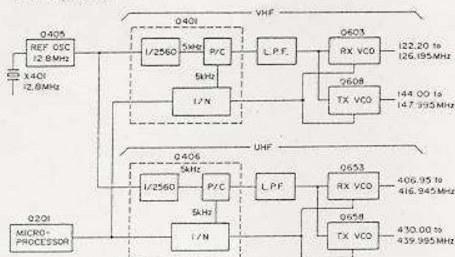
4.2 PLL Synthesizer
